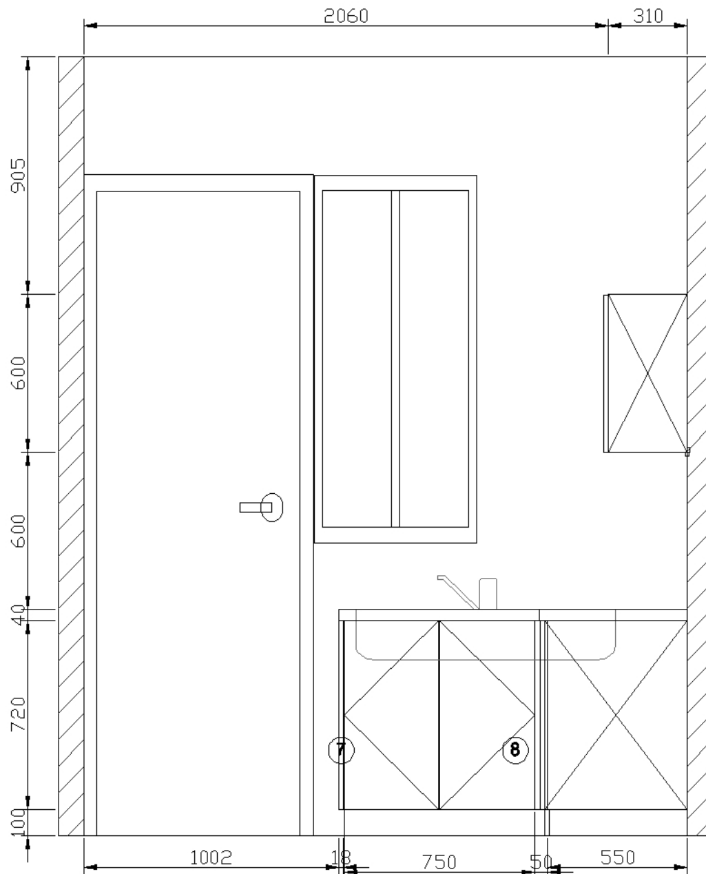
C View elevation drawing
