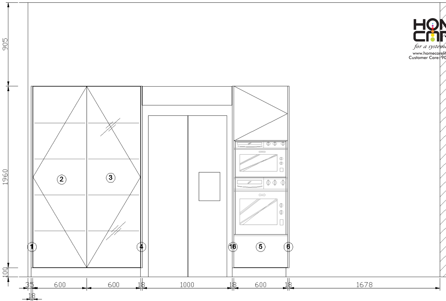
B View elevation drawing
